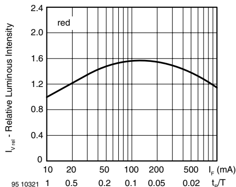
Figure 7. Rel. Luminous Intensity vs. Forw. Current/Duty Cycle
