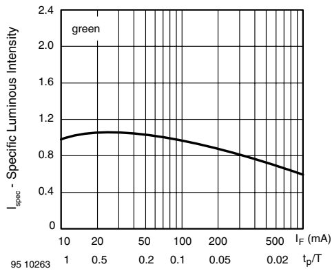
Figure 22. Specific Luminous Intensity vs. Forward Current
