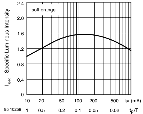
Figure 12. Rel. Lumin. Intensity vs. Forw. Current/Duty Cycle
